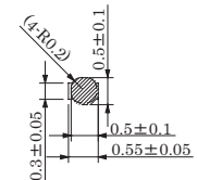
Recommended mounting hole (component-side view) *Please use 1.6mm thick PC board.
